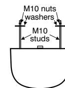
underside view
