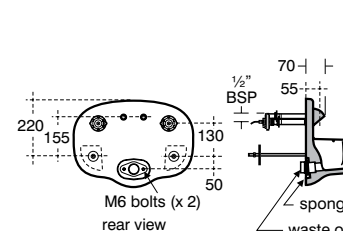
rear view
